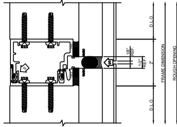
649 EXPANSION VERTICAL SERIES: 433 OUTSIDE SET SCREW SPLINE
