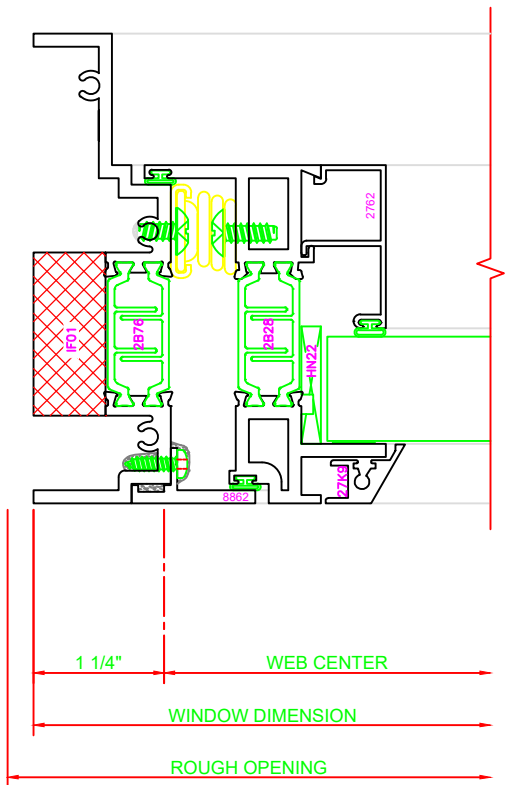
411 JAMB SERIES: 450G PROJECT IN 4-BAR ARMS
