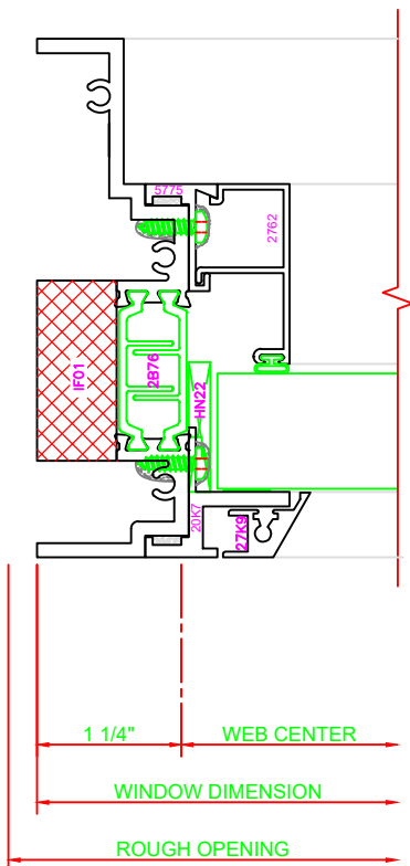
402 JAMB SERIES: 450G FIXED
