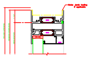
131 HEAD 201
