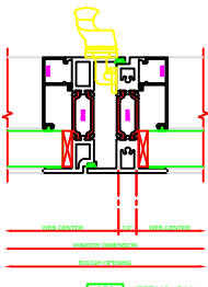
432 MEETING RAIL 201
