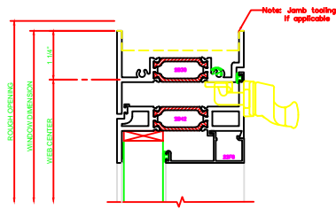
110 HEAD 325 PROJECT III CW LOCK
