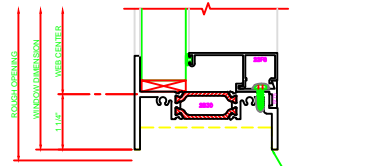
201 SILL 325 FIXED | CASEMENT III
