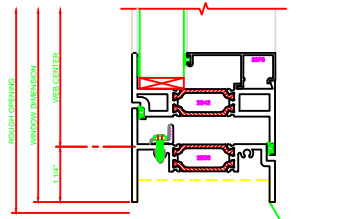
210 SILL 325 PROJECT III 4-SW. ARMS
