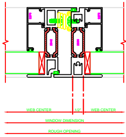
611 MEETING RAIL 325 P.A. | FIXED
