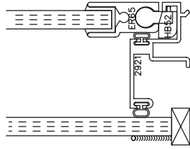
ER65 - 1/4" INTERIOR PANEL 1/4" GLAZE
