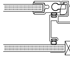
ER65 - 1/4" INTERIOR PANEL 1/4" GLAZE
