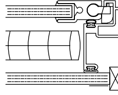
ER65 - 1/4" INTERIOR PANEL 1/4" GLAZE 5/8" BLIND
