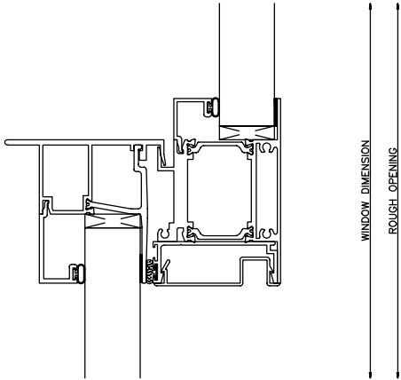
600 MEETING RAIL
