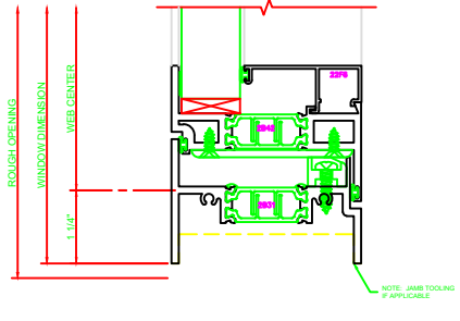
231 SILL 325 CASEMENT IN BUTT HINGES
