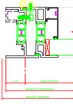
432 JAMB 325 CASEMENT IN BUTT HINGES
