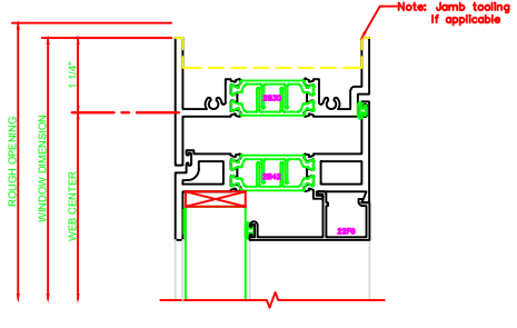
131 HEAD 325 CASEMENT IN BUTT HINGES
