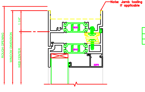
130 HEAD 325 CASEMENT IN 4-BAR ARM
