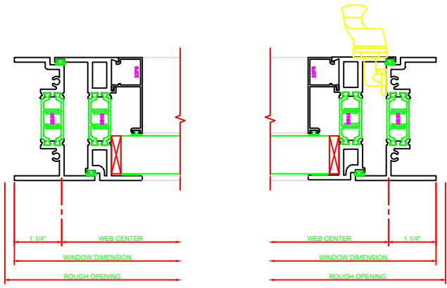
430 JAMB 325 CASEMENT IN 4-BAR ARMS ERECTOR NOTE: THE HINGED JAMB FRAME SHALL BE INSTALLED PLUMB. ALL HINGES SHALL BE SECURELY BLOCKED AND ANCHORED TO THE CONDITION THROUGH THE HINGES OR AS CLOSE AS POSSIBLE TO THE HINGES.
