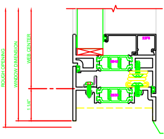
230 SILL 325 CASEMENT IN 4-BAR ARMS
