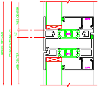
531 MEETING RAIL 325 FIXED \ CASEMENT IN BUTT HINGES
