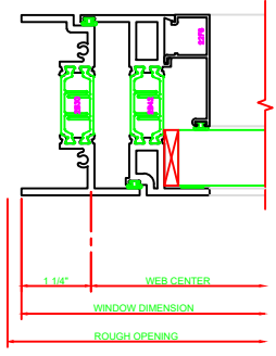
430 JAMB 325 CASEMENT IN ERECTOR NOTE: THE HINGED JAMB FRAME SHALL BE INSTALLED PLUMB. ALL HINGES SHALL BE SECURELY BLOCKED AND ANCHORED TO THE CONDITION THROUGH THE HINGES OR AS CLOSE AS POSSIBLE TO THE HINGES.
