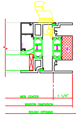
431 JAMB 325 CASEMENT IN CAM LOCK
