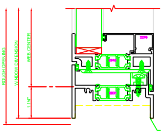
231 SILL 325 CASEMENT IN BUTT HINGES
