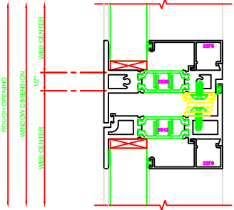
530 MEETING RAIL 325 FIXED \ CASEMENT IN 4-BAR ARMS
