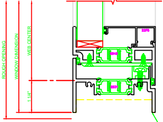
231 SILL 325 CASEMENT IN BUTT HINGES
