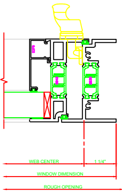
431 JAMB 325 CASEMENT IN CAM LOCK
