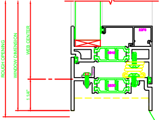
230 SILL 325 CASEMENT IN 4-BAR ARMS
