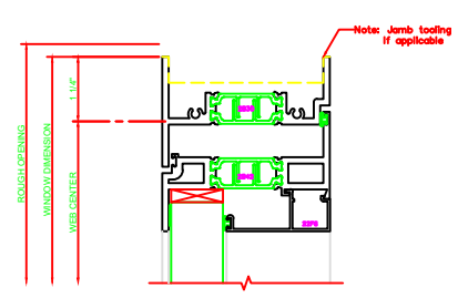
131 HEAD 325 CASEMENT IN BUTT HINGES
