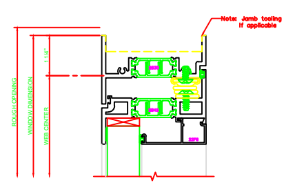
130 HEAD 325 CASEMENT IN 4-BAR ARMS
