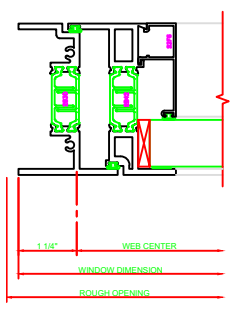
430 JAMB 325 CASEMENT IN BUTT HINGES ERECTOR NOTE: THE HINGED JAMB FRAME SHALL BE INSTALLED PLUMB. ALL HINGES SHALL BE SECURELY BLOCKED AND ANCHORED TO THE CONDITION THROUGH THE HINGES OR AS CLOSE AS POSSIBLE TO THE HINGES.
