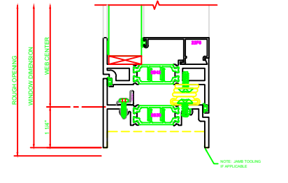
230 SILL 325 CASEMENT IN 4-BAR ARM
