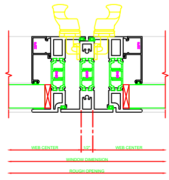
630 MEETING RAIL 325 C.L. CAM LOCK
