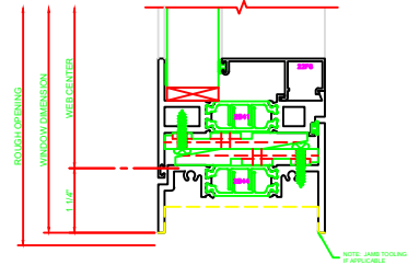
241 SILL 325 CASEMENT OUT BUTT HINGES
