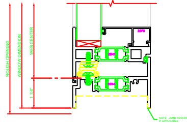
240 SILL 325 CASEMENT OUT 4-BAR ARMS
