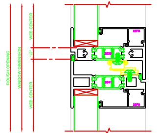
541 MEETING RAIL 325 FIXED \ CASEMENT OUT BUTT HINGES
