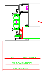
403 JAMB 325 FIXED \ CASEMENT OUT 4-BAR ARMS ERECTOR NOTE: THE JAMB SHALL BE SECURELY BLOCKED AND ANCHORED TO THE CONDITION THROUGH THE WINGS OR AS CLOSE AS POSSIBLE TO THE HINGES.
