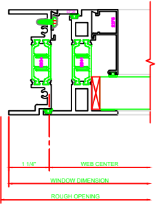
444 JAMB 325 FIXED \ CASEMENT OUT 4-BAR ARMS
