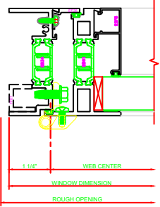
446 JAMB 325 FIXED \ CASEMENT OUT BUTT HINGES
