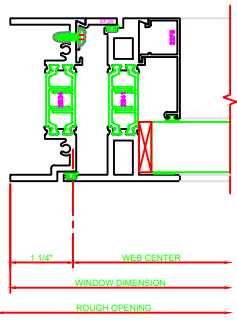
444 JAMB 325 FIXED \ CASEMENT OUT ERB CHINA NOTE: THE HINGED JAMB FRAME SHALL BE INSTALLED PLUMB. ALL HINGES SHALL BE SECURELY BLOCKED AND ANCHORED TO THE CONDITION THROUGH THE HINGES OR AS CLOSE AS POSSIBLE TO THE HINGES.
