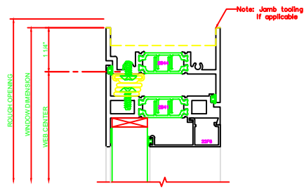
140 HEAD 325 CASEMENT OUT 4-BAR ARM
