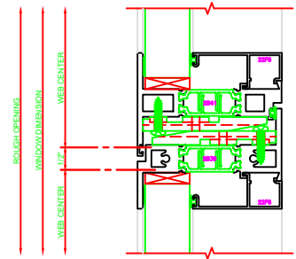
543 MEETING RAIL 325 CASEMENT OUT \ FIXED BUTT HINGES
