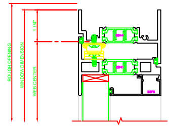
141 HEAD 325 CASEMENT OUT BUTT HINGES
