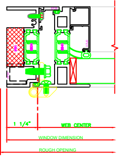
446 JAMB 325 FIXED \ CASEMENT OUT BUTT HINGES
