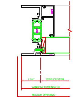
403 JAMB 325 PROJECT OUT \ FIXED
