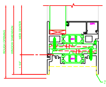
241 SILL 325 CASEMENT OUT BUTT HINGES
