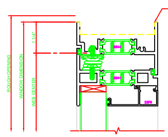
140 HEAD 325 CASEMENT OUT 4-BAR ARM
