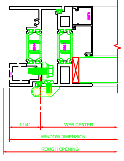
442 JAMB 325 CASEMENT OUT BUTT HINGES
