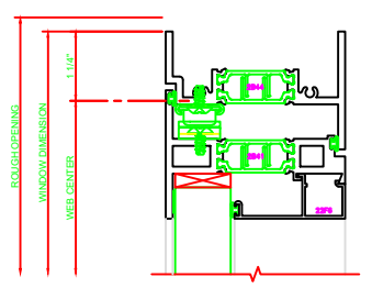
141 HEAD 325 CASEMENT OUT BUTT HINGES
