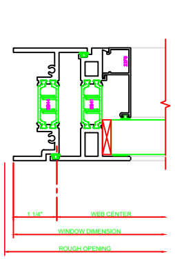
440 JAMB 325 CASEMENT OUT 4-BAR ARM RECHECK NOTE: THE FINISHED JAMB FRAME SHALL BE INSTALLED PLUMB. ALL HINGES SHALL BE SECURELY BLOCKED AND ANCHORED TO THE CONDITION THROUGH THE HINGES OR AS CLOSE AS POSSIBLE TO THE HINGES.
