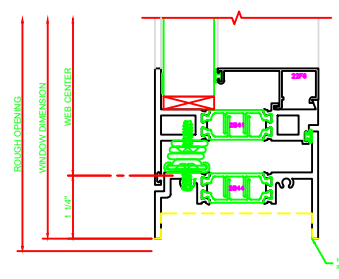
240 SILL 325 CASEMENT OUT 4-BAR ARMS
