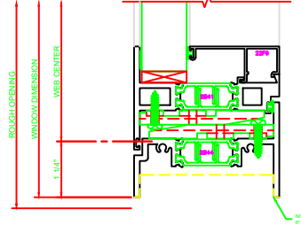
241 SILL 325 CASEMENT OUT BUTT HINGES
