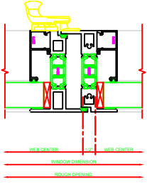
642 MEETING RAIL 250 CASSETTE OUT | PSED ON LOCK
