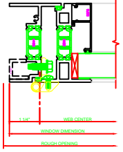
442 JAMB 250 CASSETTE OUT BUT PSED
