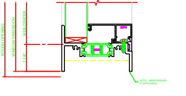
201 SILL 325 FIXED | CASEMENT IN
