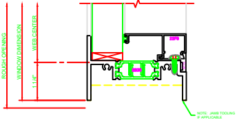
201 SILL 325 FIXED | CASEMENT IN
