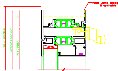
110 HEAD 325 PROJECT IN OW LOCK
