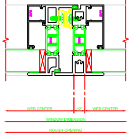
611 MEETING RAIL 325 P.L. | FIXED
