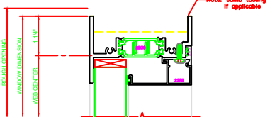
101 HEAD 325 FIXED | PROJECT IN
