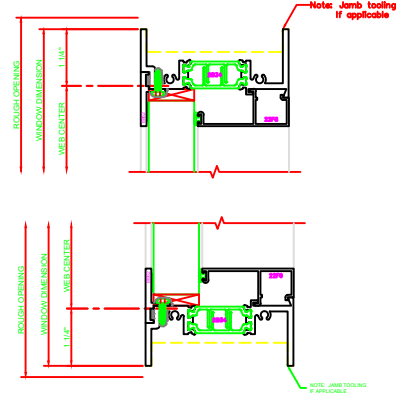
102 HEAD 325 FIXED | CASEMENT OUT
