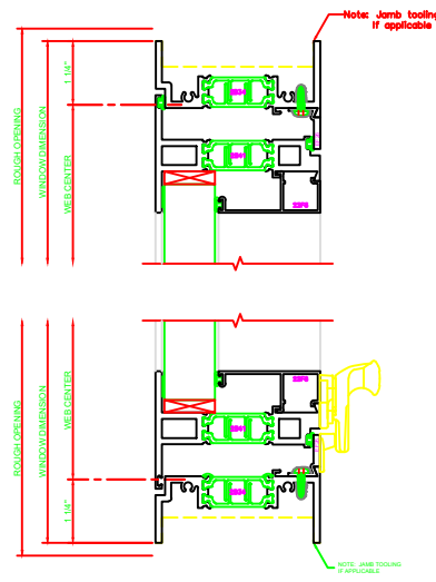
121 HEAD 325 PROJECT OUT | FIXED 4-BAR ARMS
