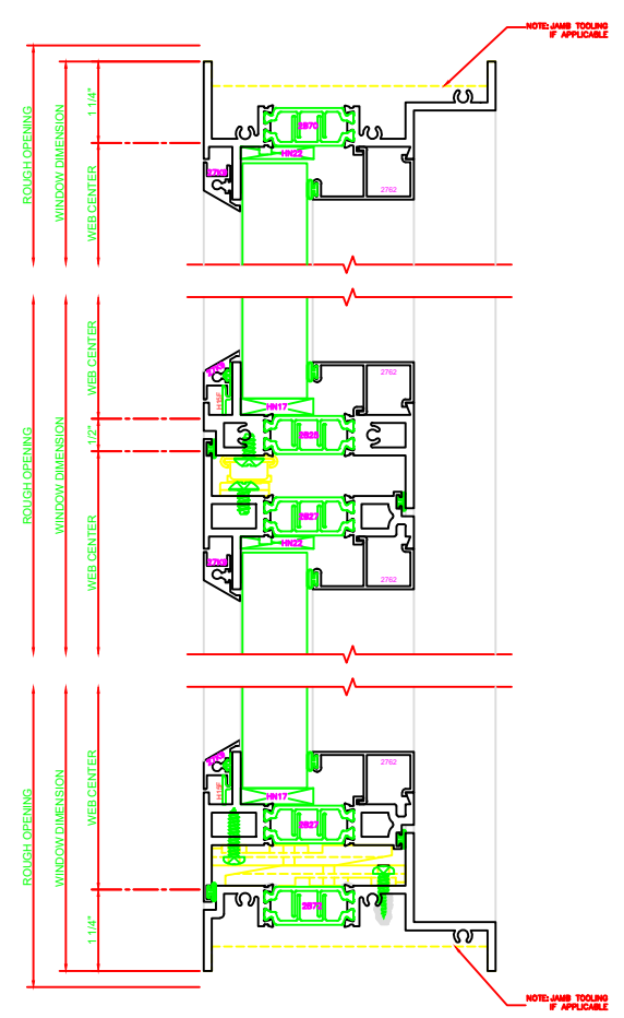
541 MEETING RAIL SERIES: 450G FIXED/C.O. BUTT HINGE
