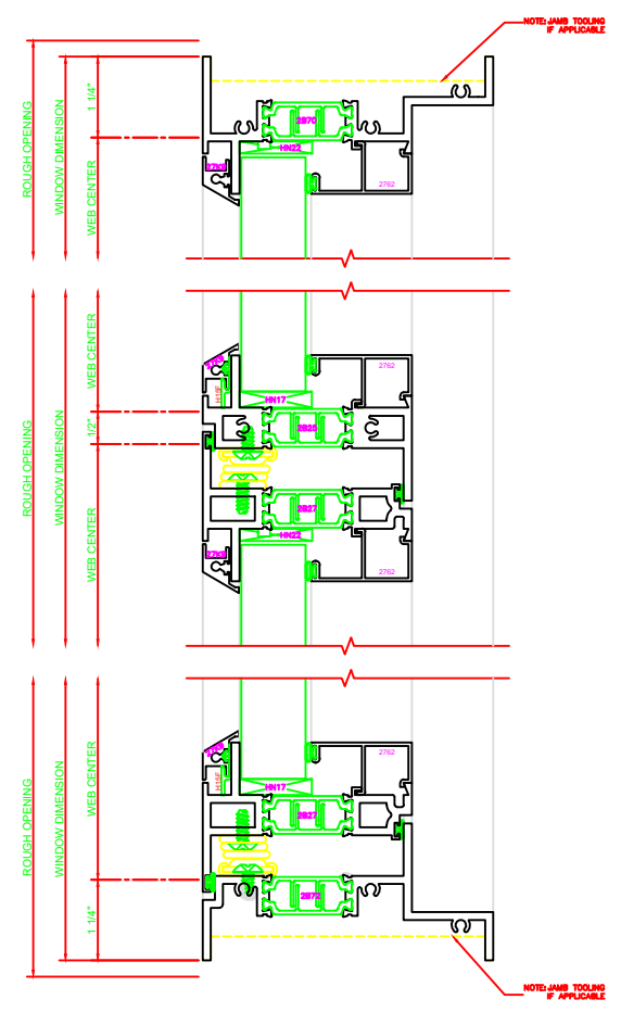
540 MEETING RAIL SERIES: 450G FIXED/C.O. 4-BAR ARMS
