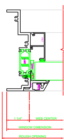
403 JAMB SERIES: 450G FIXED
