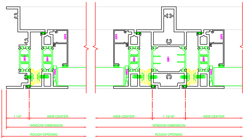
420 JAMB SERIES: 450X PROJECT OUT 4-BAR ARMS
