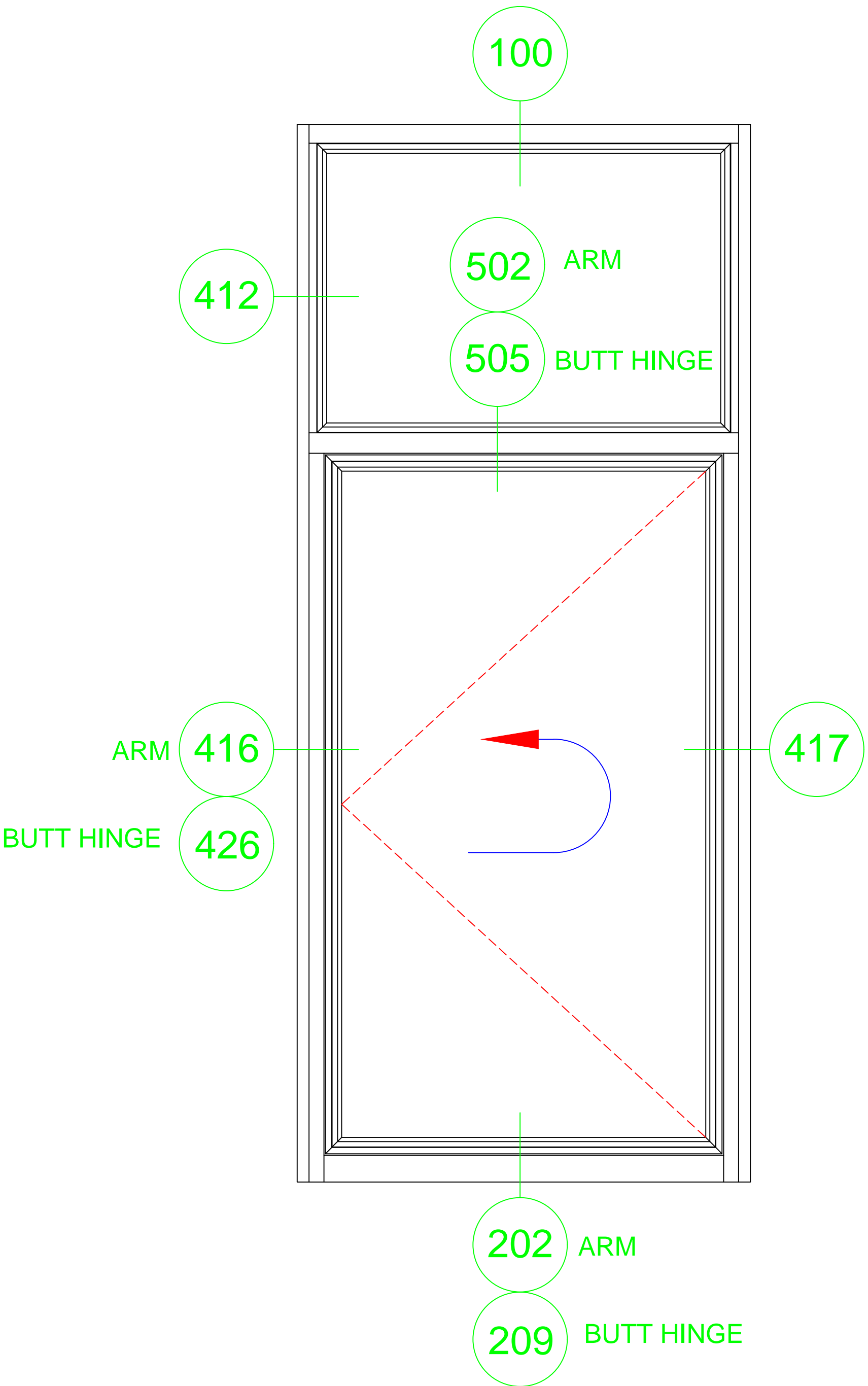
S550G INSIDE GLAZED FIXED/CASEMENT IN LEFT BUTT HINGES AND CASEMENT ARMS
