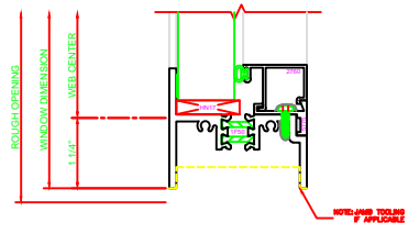
201 SILL SERIES: 5501 FIXED
