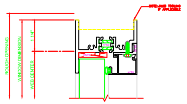
101 HEAD SERIES: 5501 FIXED
