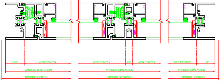
410 JAMB SERIES: 5501 PROJECT IN 4-BAR ARMS
