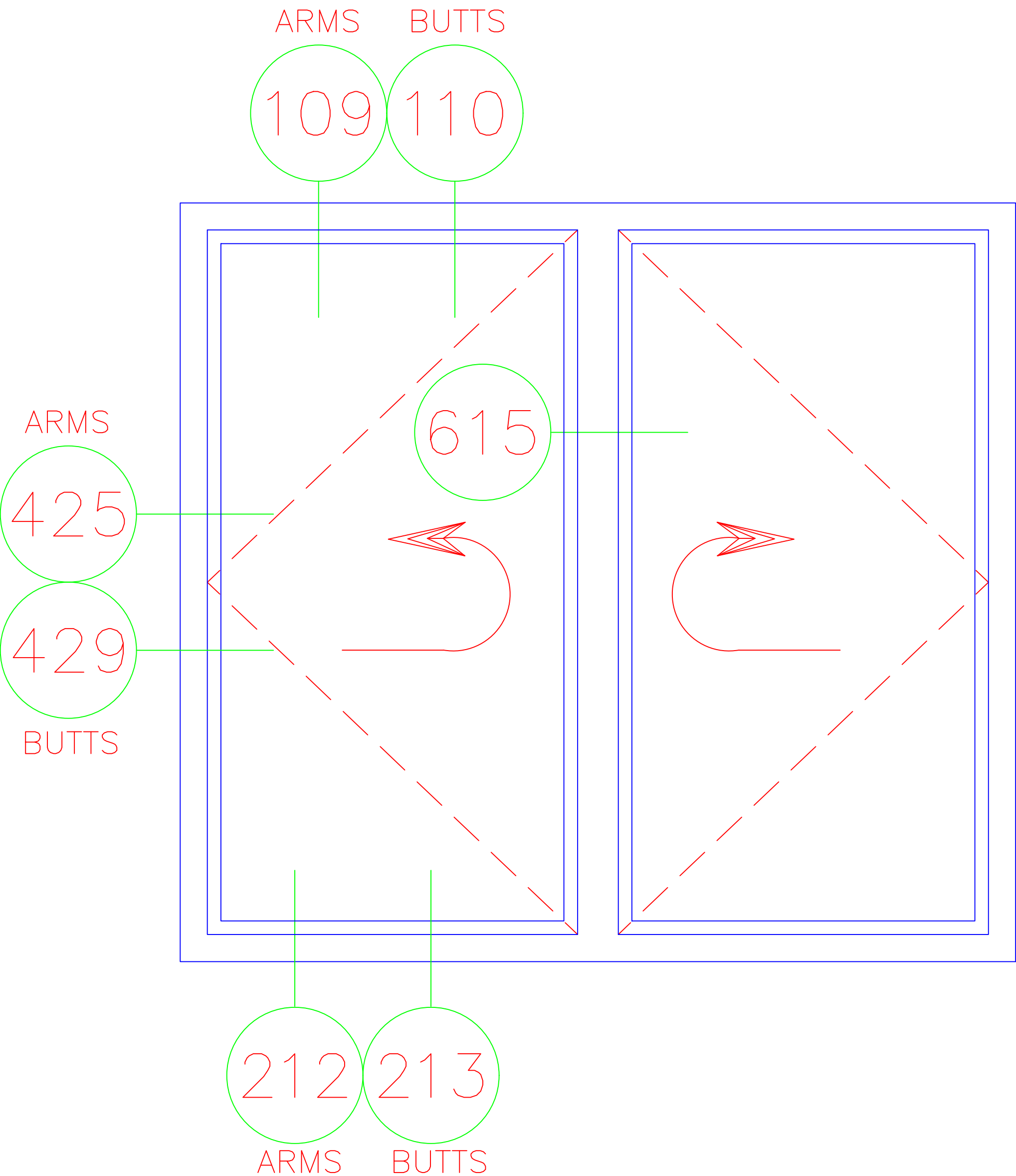
810i Inside Glazed Casement In Beside Casement In Left Swing and Right Swing 4-Bar Arms / Butt Hinges Cam Locks
