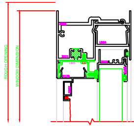
100 HEAD SERIES: 3500
