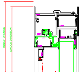
100 HEAD SERIES: 3500
