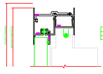
101 HEAD SERIES 3000
