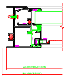
411 JAMB SERIES 3000
