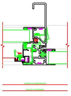
606 MEETING RAIL SERIES 3000
