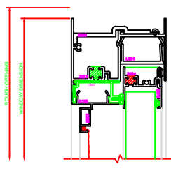
104 HEAD SERIES 3000
