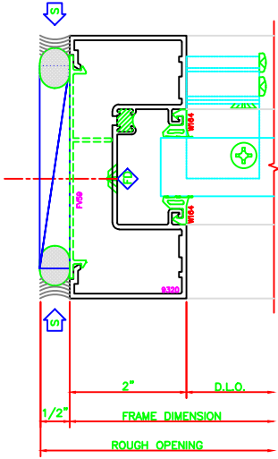
402 JAMB 403 SHEARBLOCK
