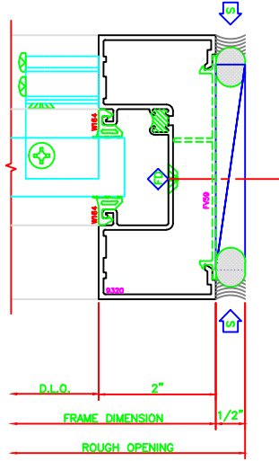
403 JAMB 403 SHEARBLOCK
