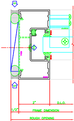
402 JAMB 403 SHEARBLOCK
