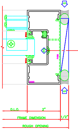
403 JAMB 403 SHEARBLOCK
