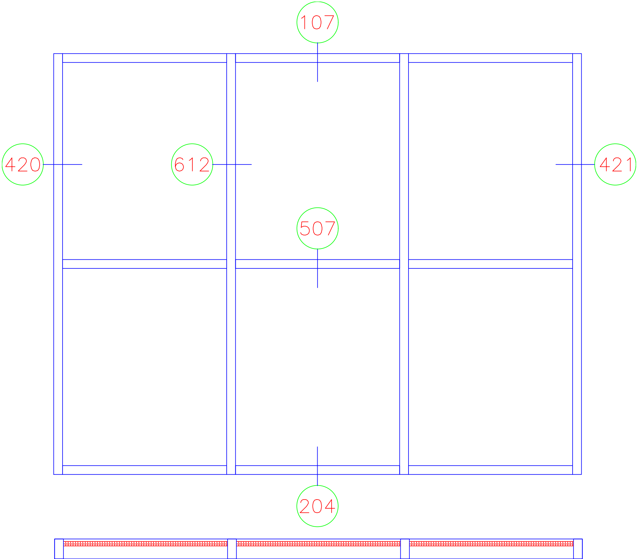
S433 Inside Glazed Inside Set 2" x 4 1/2" Screw Spline
