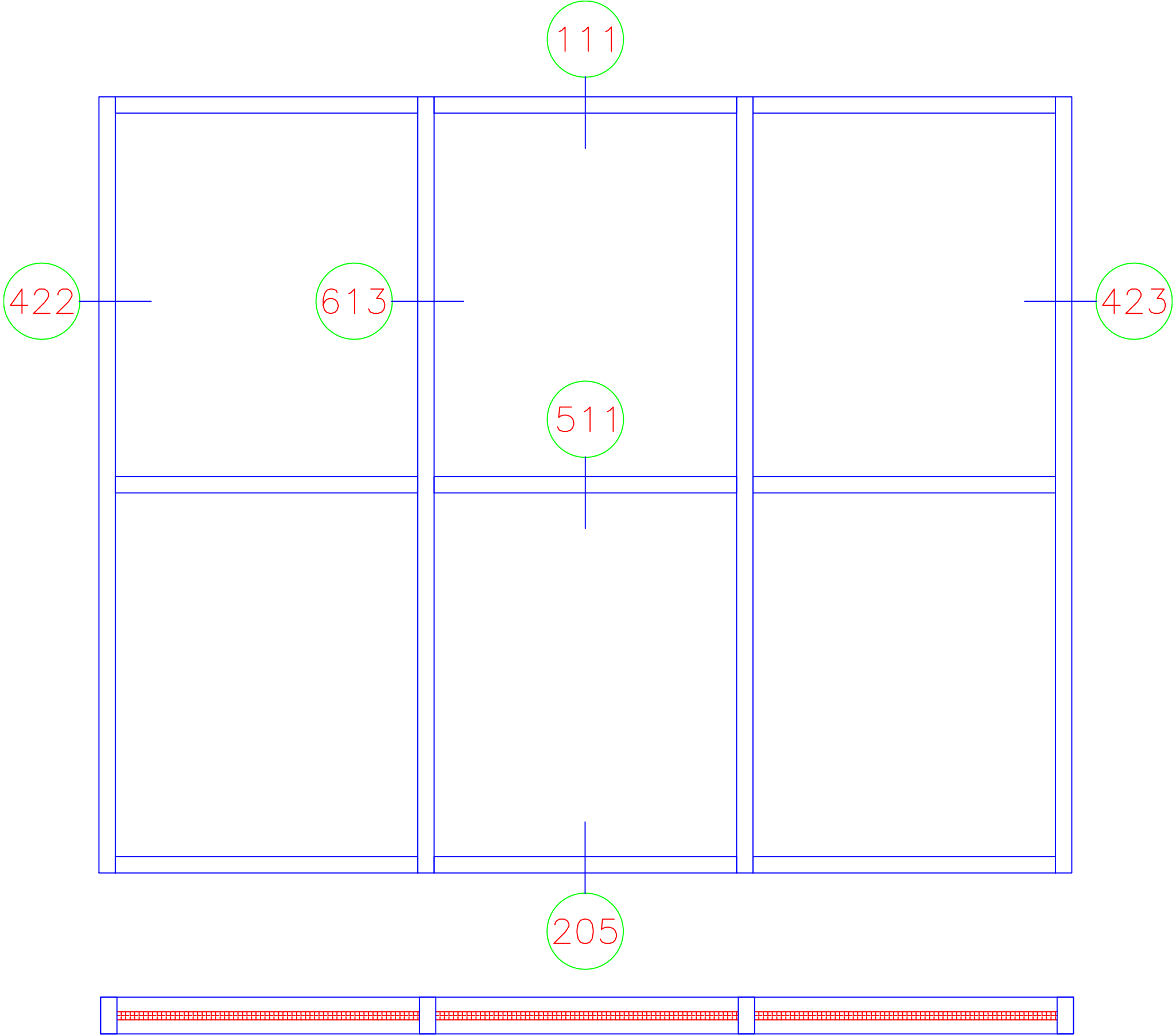
S433 Inside Glazed Center Set 2" x 4 1/2" Screw Spline
