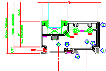
200 SILL S433
