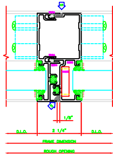
648 EXPANSION VERTICAL S433 SPARELOCK
